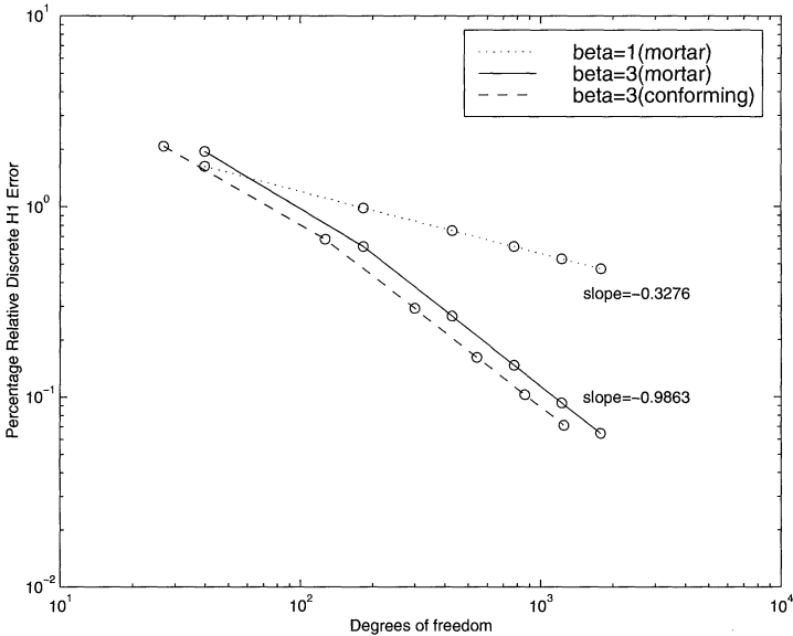
FIGURE 3. The relative error in the energy norm in dependence on h for radical meshes ( k = 2 )
