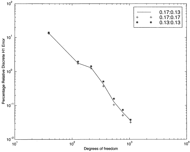
FIGURE 5. Comparison of the p version mortar and conforming FEMs for n = 4
