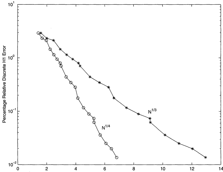
FIGURE 6. Exponential convergence for the hp mortar FEM
